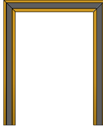
NAME - FRAME - INLAY - FRM20 FINISH - BRASS / BLACK FPF PART NO. - F800068 PARTS CENTER PART NO. TBA
